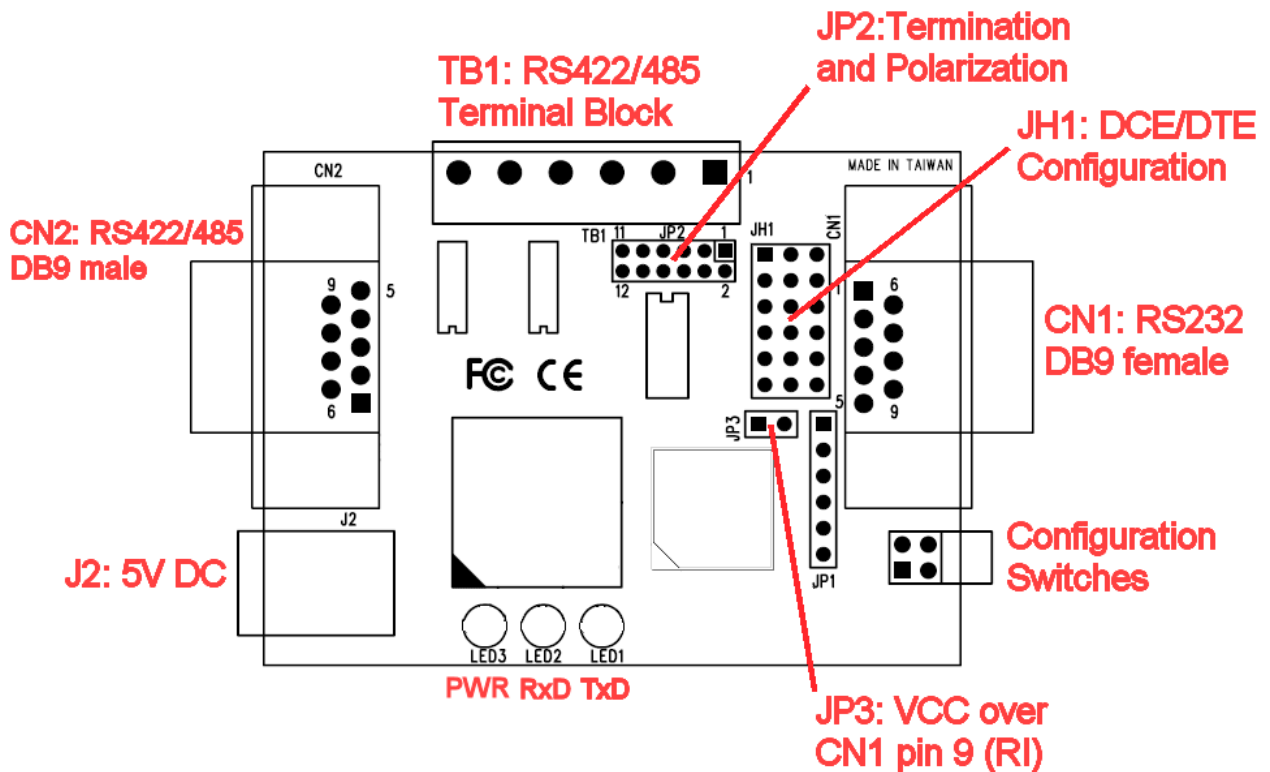
Figure 1: Internal view of SER-485 Lite
