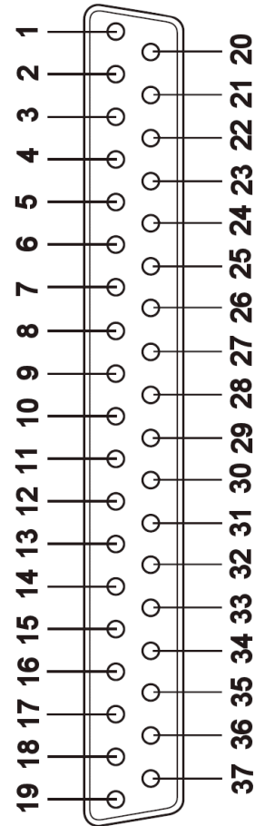
Figure 29: DB37 female Connector
