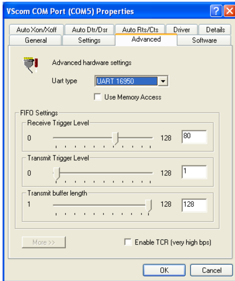
Figure 18: Advanced Settings 16C950
