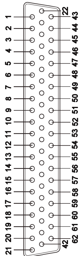
Figure 28: DB62 female Connector
