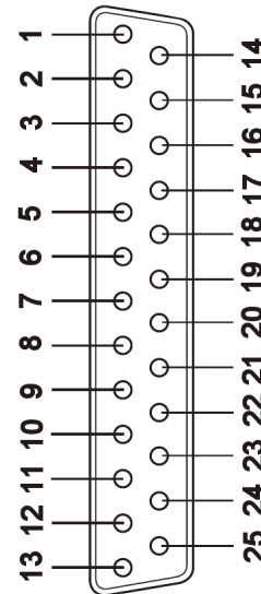
Figure 32: DB25 female LPT
