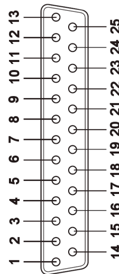
Figure 31: DB25 male RS 232
